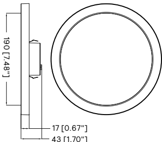
Surface Mount Downlight 9"
