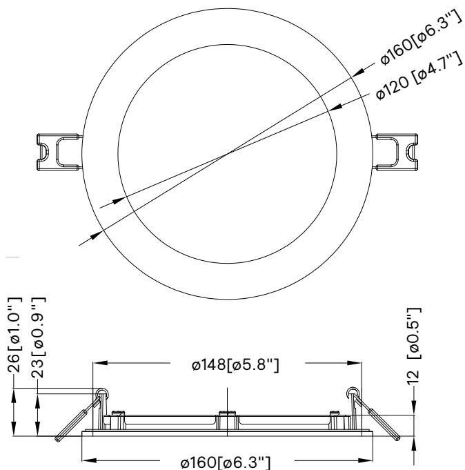
Downlight 5" Round
