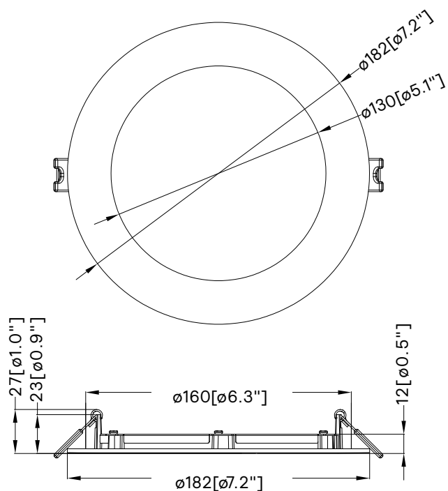
Downlight 6" Round
