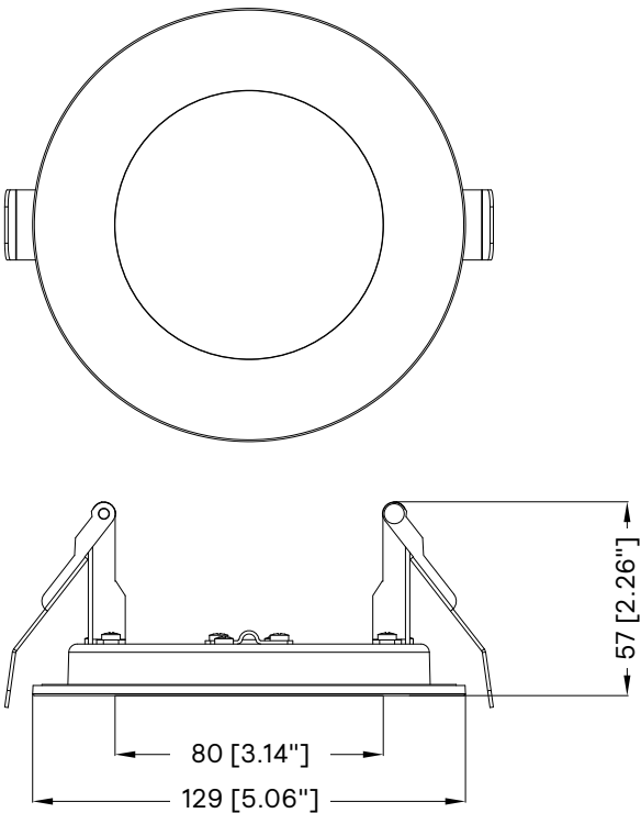
Downlight 4" Round
