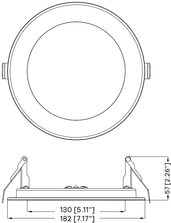
Downlight 6" Round
